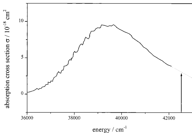
FIG. 1. Absorption cross section of \text{CSCI}_2 (Ref. 19), the photon energy used in the present experiment is marked by an arrow. Due to the lack of experimental data, the absorption cross section in the high energy range is extrapolated and presented by a dotted curve.
