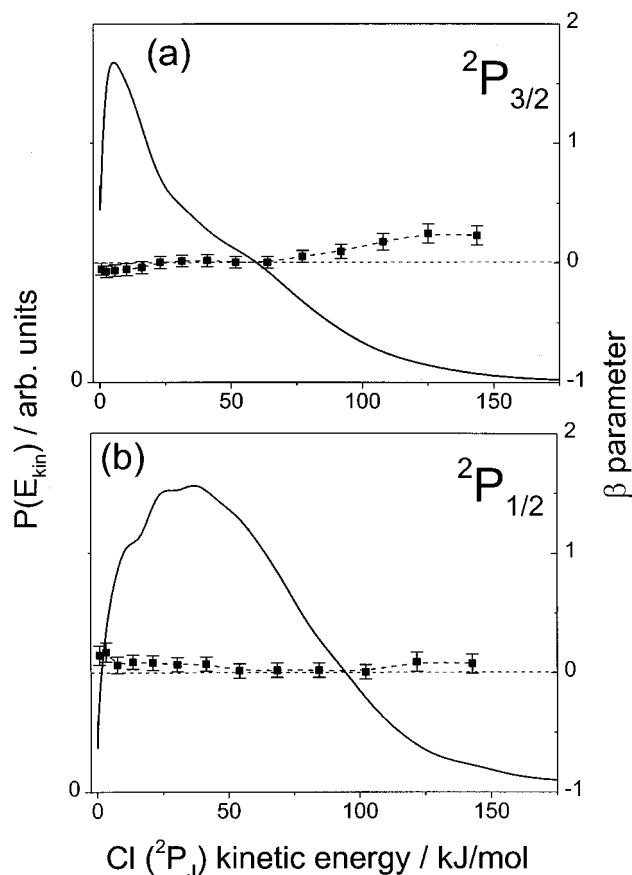
FIG. 2. Kinetic energy distribution for (a) ground state Cl( 2 P 3/2 ) and (b) excited state Cl*( 2 P 1/2 ) atoms produced in the photodissociation of CSCI 2 at 235 nm. The dependence of the β parameter on the Cl fragment kinetic energy (right scale) is shown by curves with error bars. This 1D presentation is obtained via integration of the 3D data.
